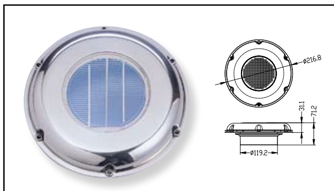
4" S.S. Solar Powered Ventilator
