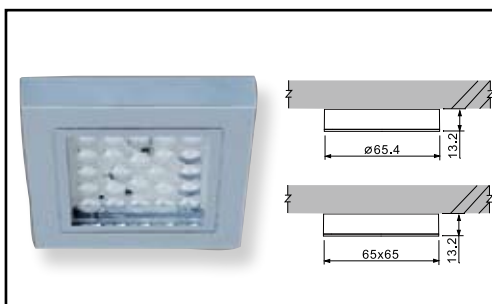
LED Ceiling Light
