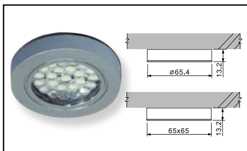
LED Ceiling Light
