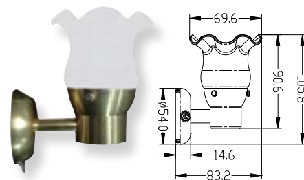
Dimmable LED Wall Reading Light
