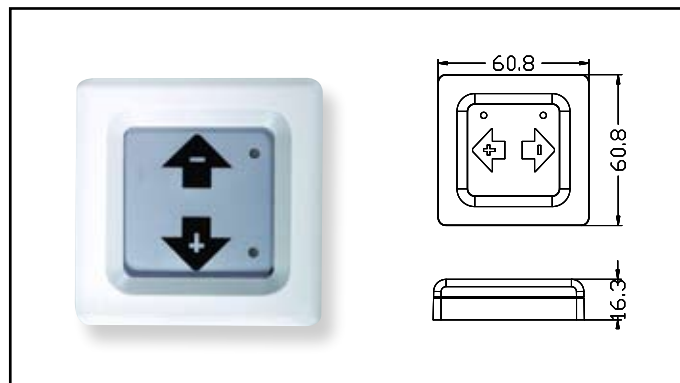
12V Dimmer Switch
