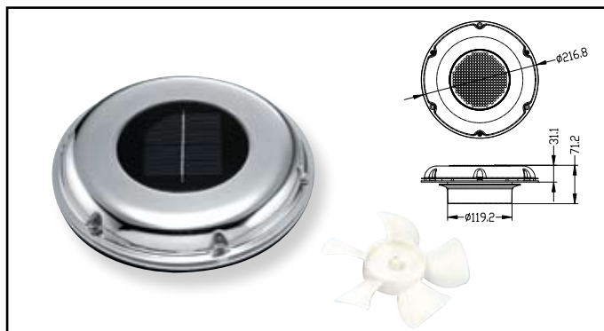
4" S.S. Solar Powered Ventilator
