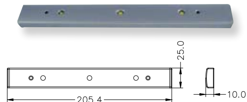
Dimmable LED High Power Strip Light
