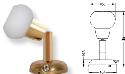
Dimmable LED Swivel Reading/Wall Light
