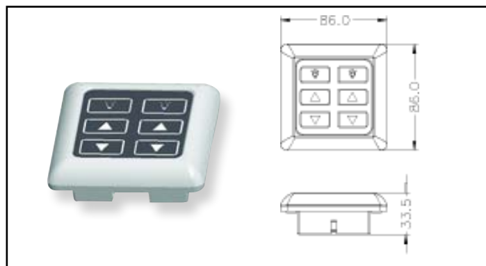
12V Dual Circuit Dimmer Switch w/ Remote Control
