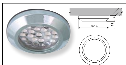
LED Ceiling Light
