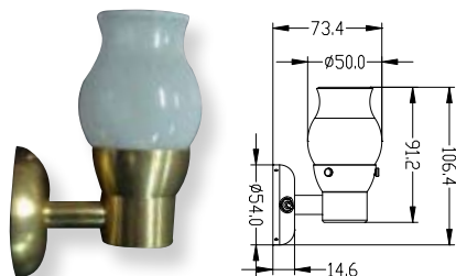
Dimmable LED Wall Reading Light
